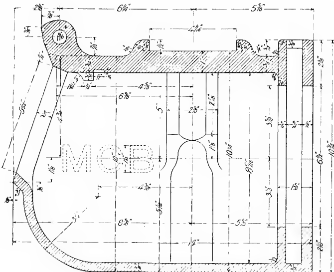
Fig. 5386. Longitudinal Section.
